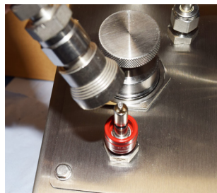
Fig. 7 Sample line to inlet connection.
