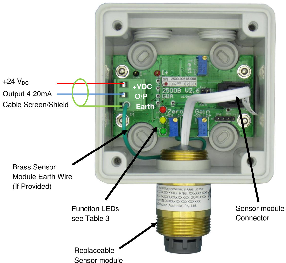
Figure 4: Sensor Wiring
