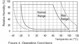
Figure 4. Operating Conditions
