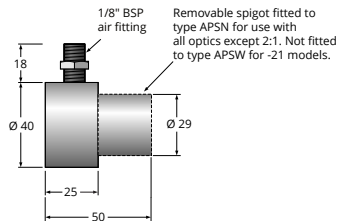
Air Purge Collar
