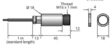
Sensing Head
