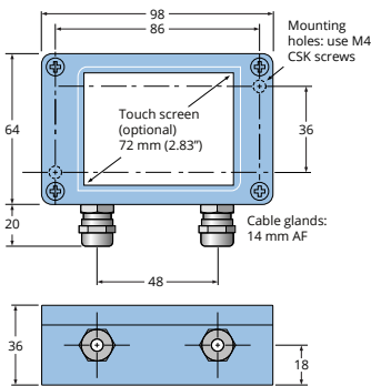
Electronics Module
